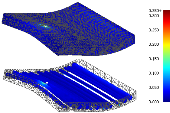
Fig. 9: A screenshot of our 3D simulation on a heterogeneous mesh with 20 veins. The maximum strain is color coded. The top image shows the triangles on the surface of the mesh. Bottom image shows the strain on the veins. The depth is expanded to 3.5cm.
