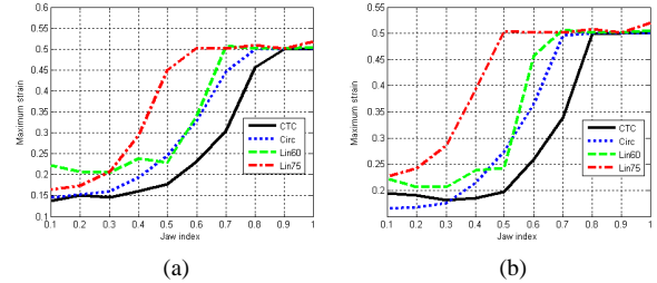
Fig. 8: Comparison between linear, circular and the CTC trajectories for two lines-of-sight, starting at distance (a) 25% and (b) 15% from the fixed end of the tissue. Each line-of-sight has 45° slope. Strain of 0.5 means failure. The CTC trajectories usually outperform the other trajectories, but circular trajectories perform slightly better for some grasp locations when the line-of-sight approaches the fixed end of the tissue.
